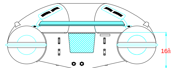
AFT VIEW VISTA TRASERA
