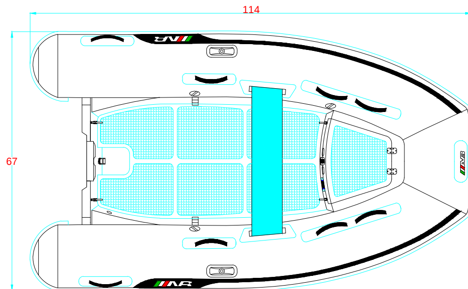
PLANT VIEW VISTA SUPERIOR
