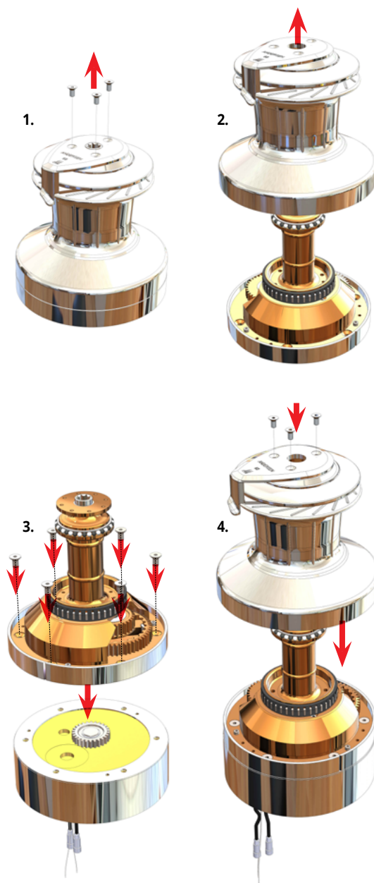
Winch installation
