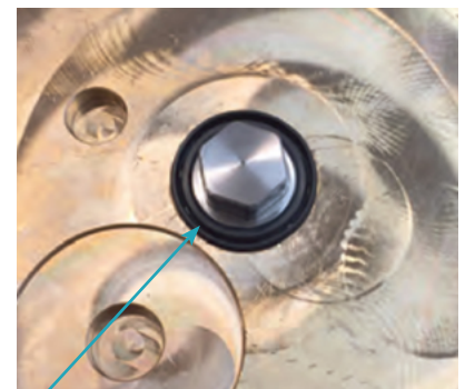
Lubrication of motor drive shaft lip seal.
