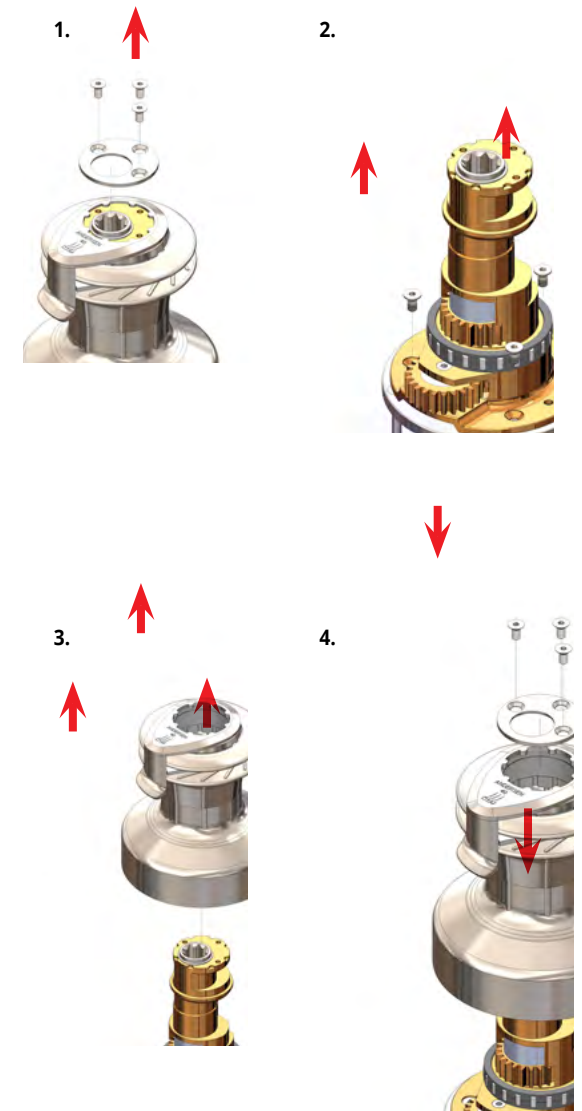
Winch installation
