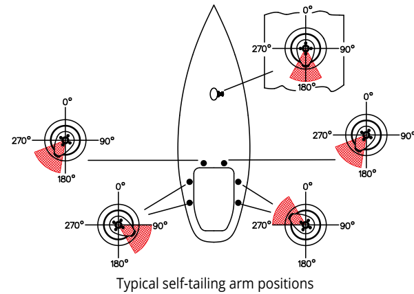
Typical self-tailing arm positions
