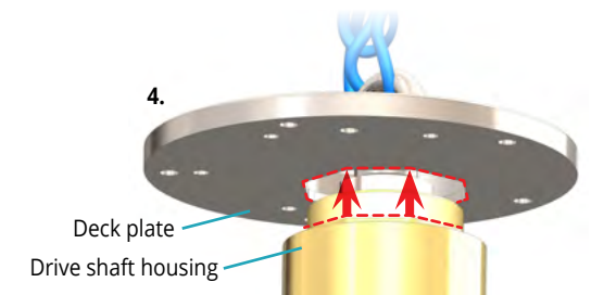
Octagonal detail on drive shaft housing mates with recess in deck plate.
