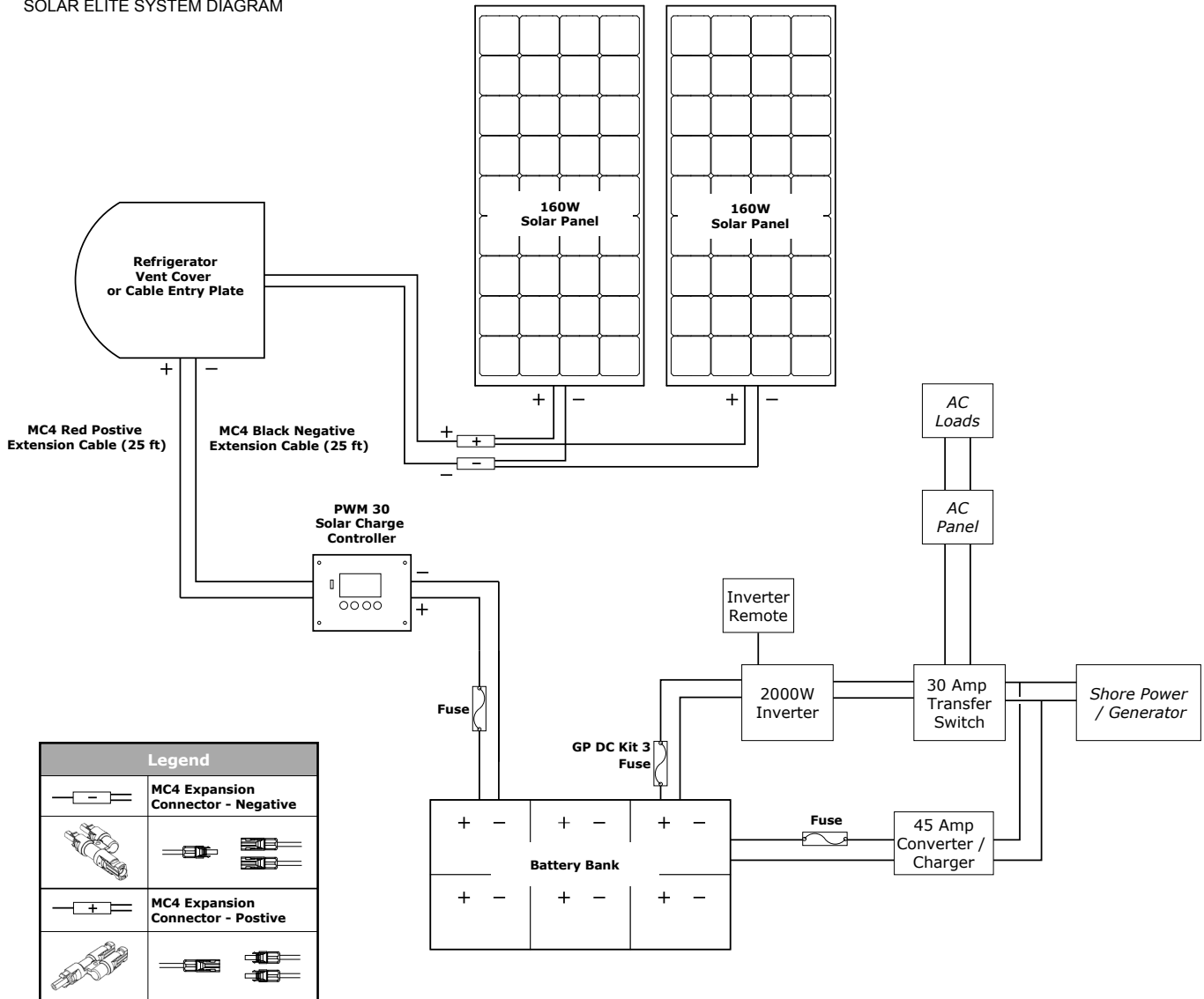
SOLAR ELITE SYSTEM DIAGRAM
