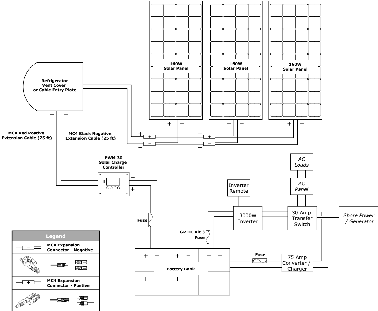
SOLAR EXTREME SYSTEM DIAGRAM
