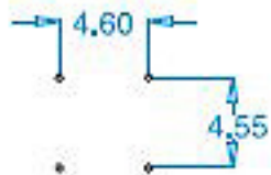
MOUNT PATTERN, FRONT
