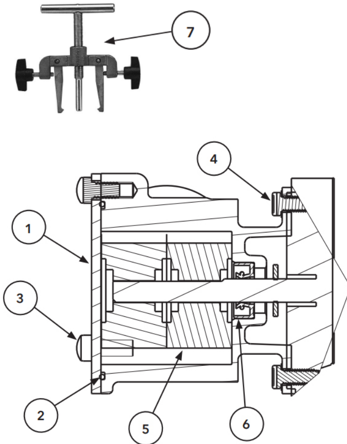
Jabsco impeller removal tool 50070-0040
