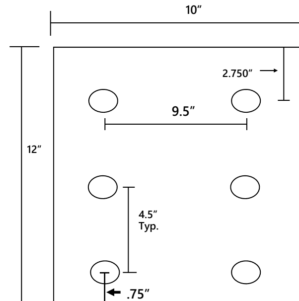
Transom Plate Hole Pattern [not to scale]
