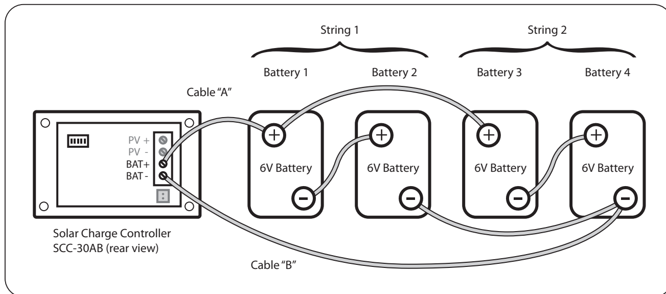
Fig. 5.3: Series-Parallel Connection
