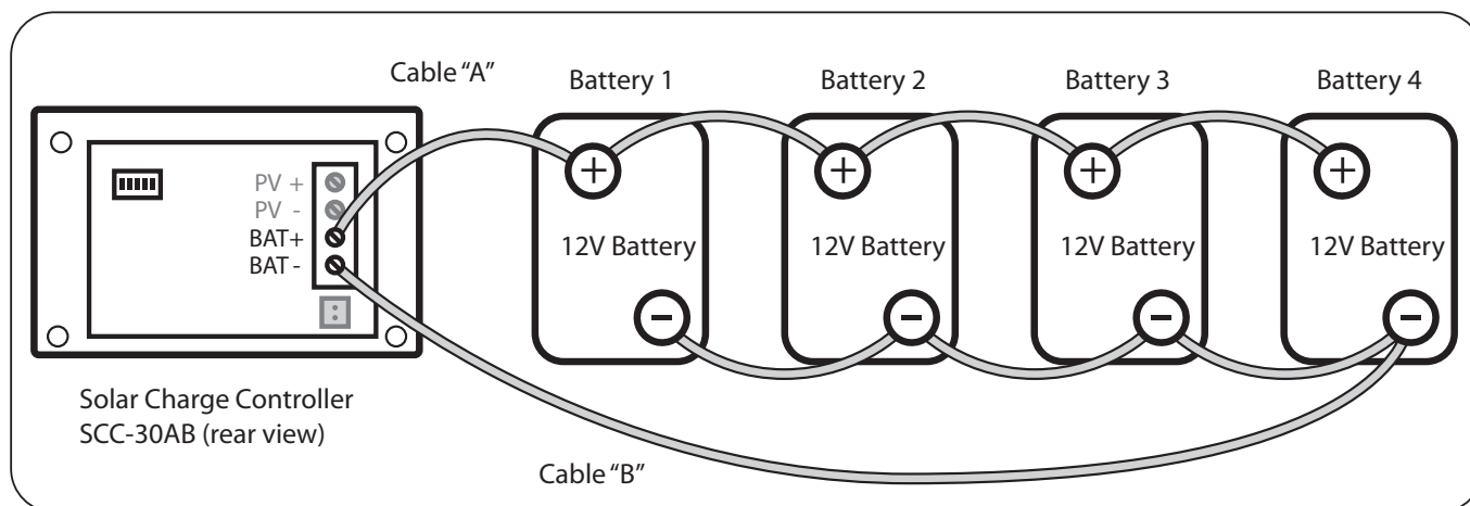
Fig. 5.2: Parallel Connection
