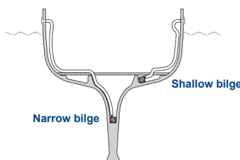
Typical Installation
