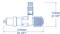
DIMENSIONS FOR 1100 MODEL Side View
